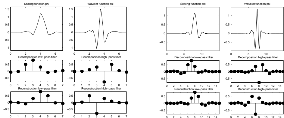
Figure 6-13: Symlets \text{sym}4 on the Left and \text{sym}8 on the Right
